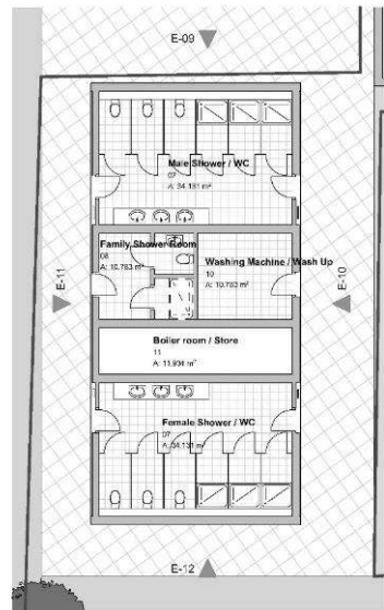
Proposed Ground Floor Plan 1:100
