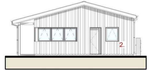
4 West - Proposed 1 : 100
