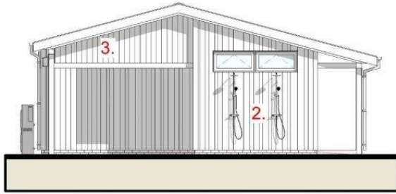
1 East - Proposed 1 : 100
